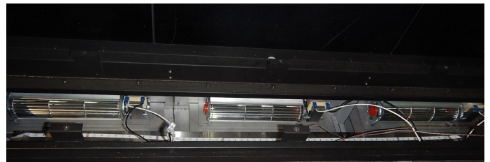
Figure 27.d secure the fans
