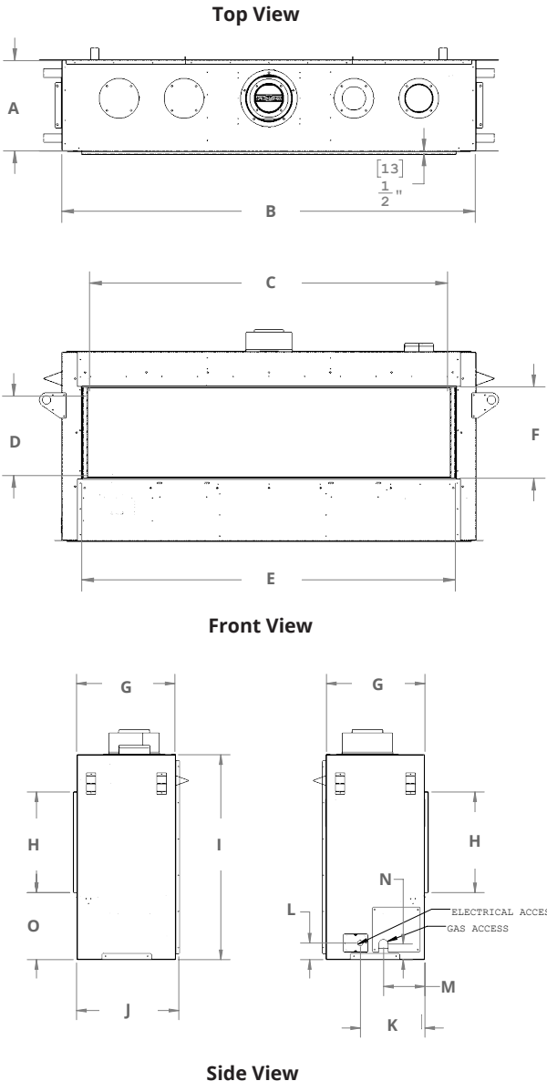
Figure 2. DL6315, D6315 Fireplace dimensions (Tolerance ± 1/8").
