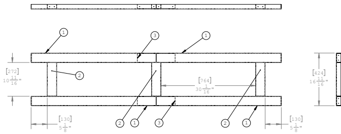
Figure 8. Assembly of Non Combustible Framing
